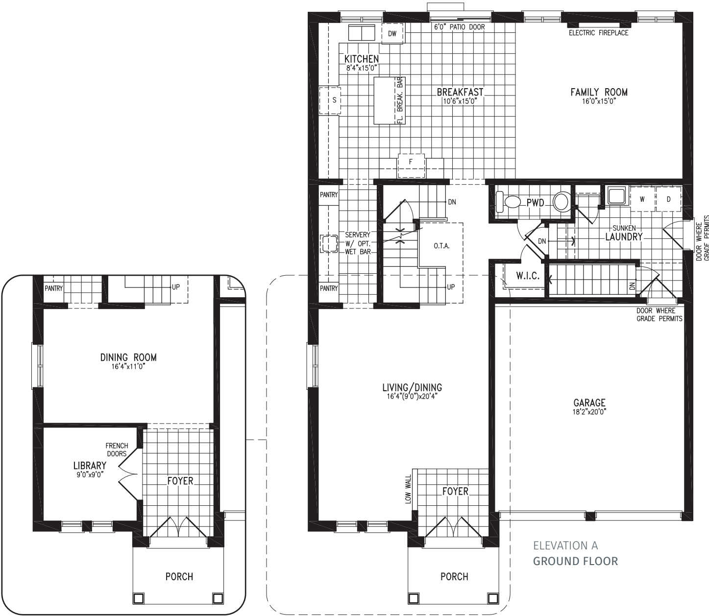
ELEVATION A OPT. LIBRARY/DINING ROOM
